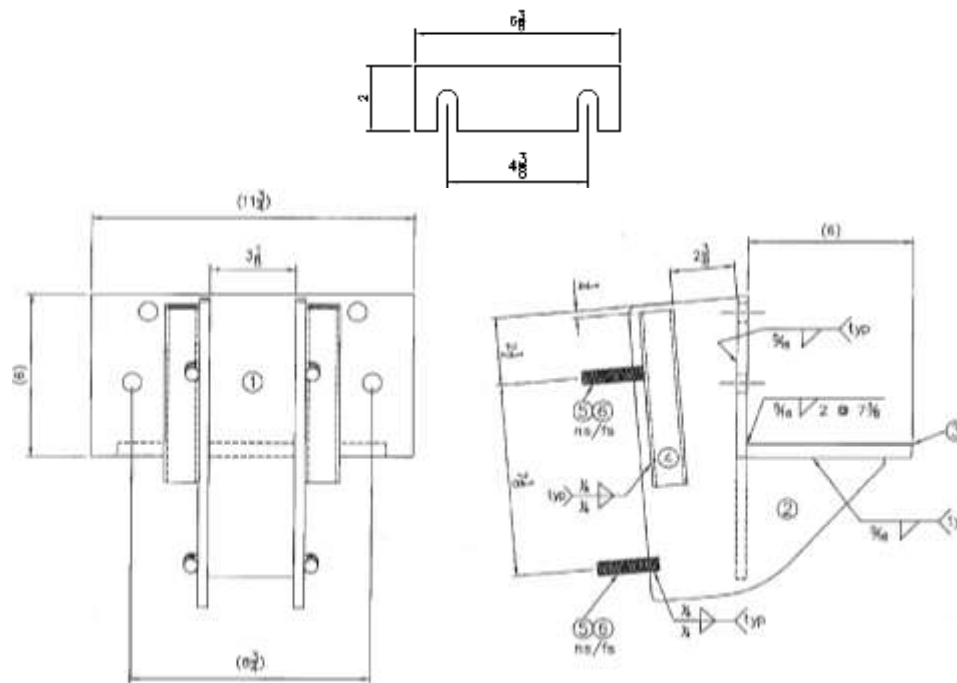
FIGURE 4—TAB-MUB BRACKETS
