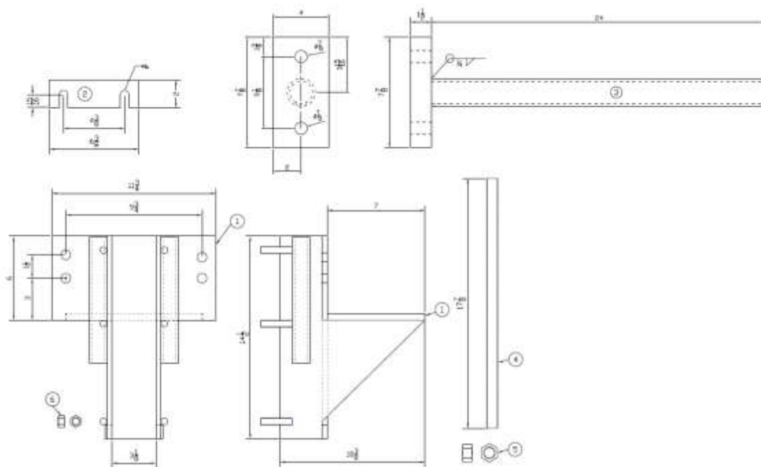
FIGURE 6—MODEL-300 BRACKET
