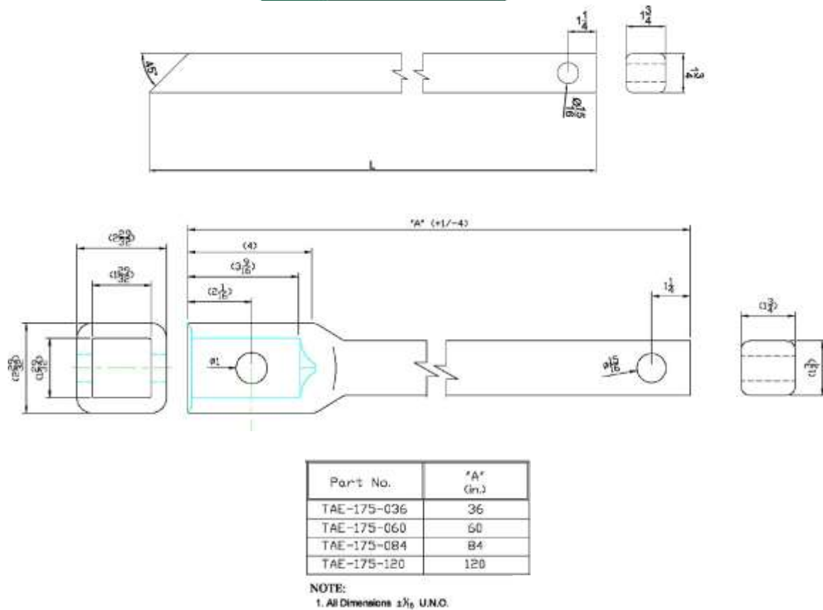
FIGURE 2B—TA-175 LEAD AND EXTENSION SECTION (COUPLER SECTION DETAIL AS SHOWN IN FIGURE 2A )
