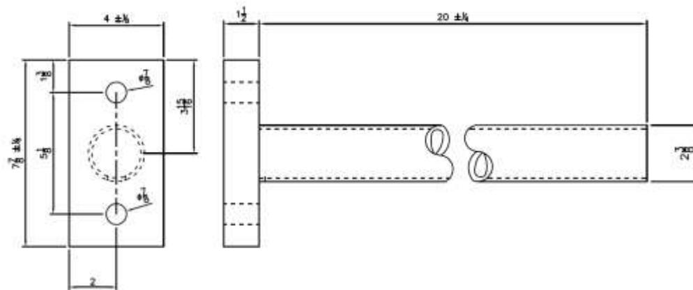
T-Tube Subassembly for the TA-150 Pile
