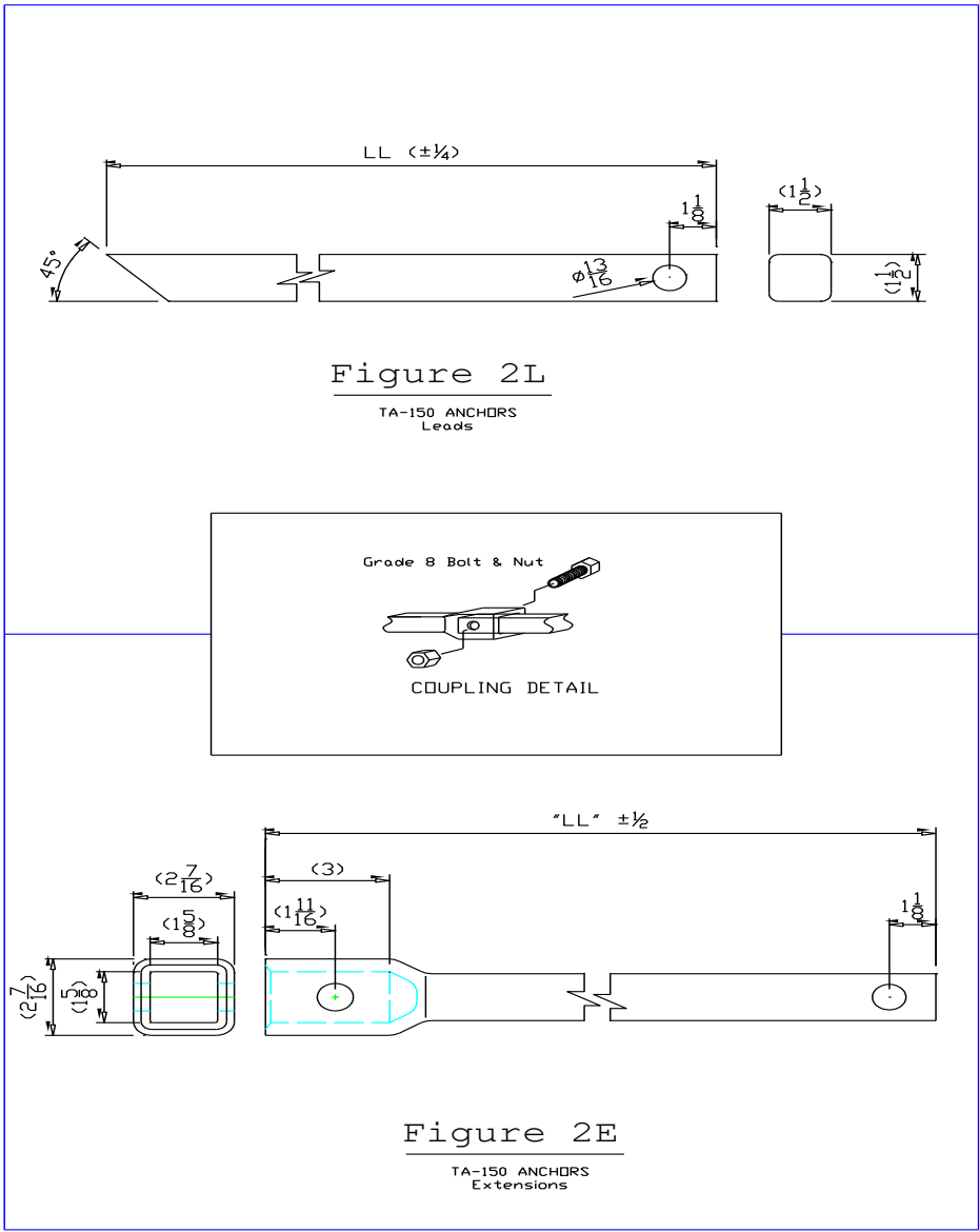
FIGURE 2A—TA-150 LEAD SECTION, COUPLER AND EXTENSION SECTION
