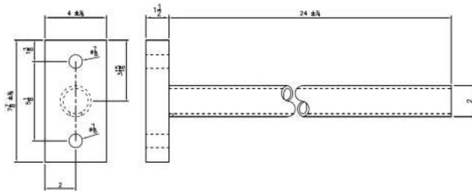
T-Tube Subassembly for the TA-288 Pile
