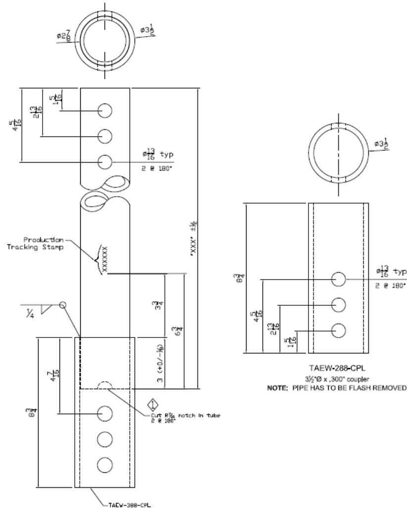
FIGURE 1A(b) – TA-288 LEAD SECTION, WELDED COUPLER AND EXTENSION SECTION (ALTERNATE)
