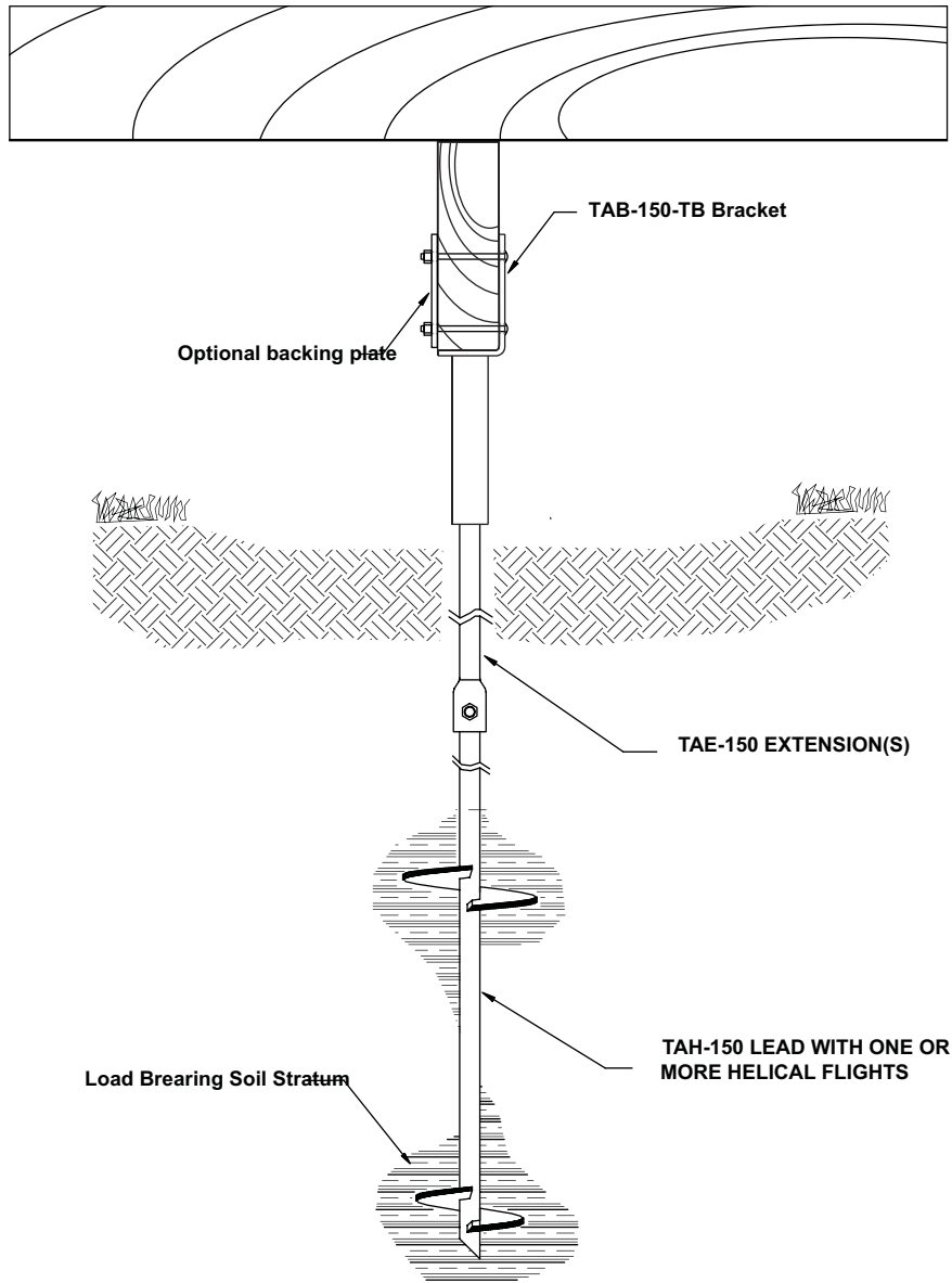
TAB-150-TB Timber Bracket Application Drawing
