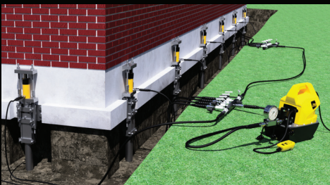
Hydraulic Lift
