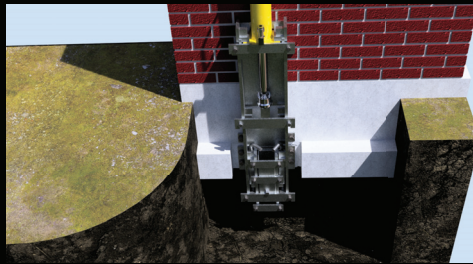
Installation
