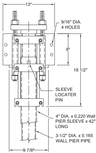
PPB-450EP2 - 2" Eccentric Utility Bracket Details
