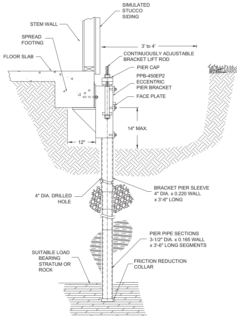
PPB-450EP2 - 2" Eccentric Utility Bracket Application Drawing
