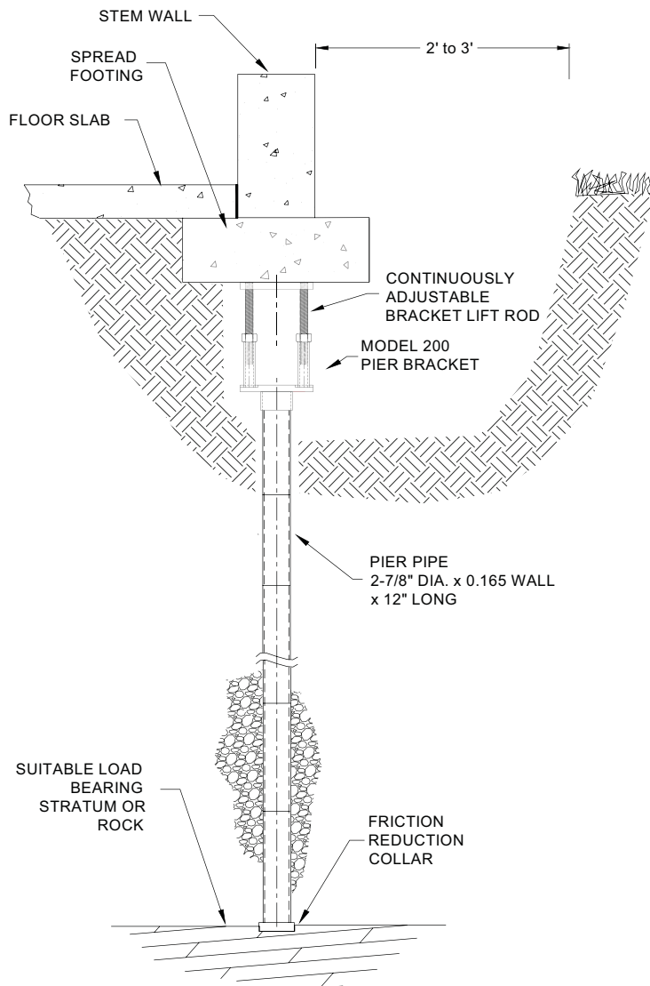
PPB-200 Utility Bracket Application Drawing
