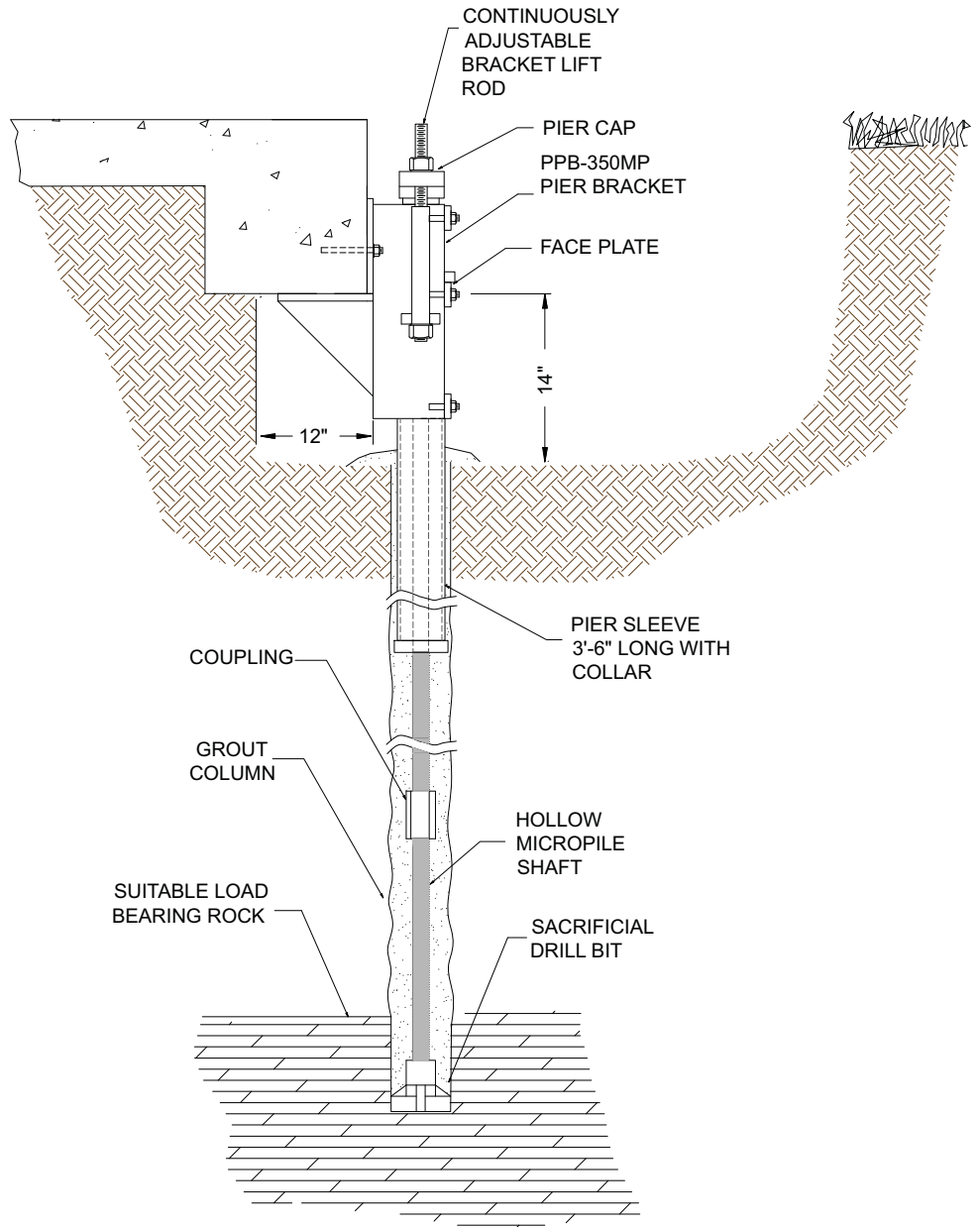
PPB-350MP –Typical Micro Pile Application Drawing
