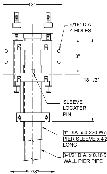
PPB-350MP Micro Pile Bracket Details
