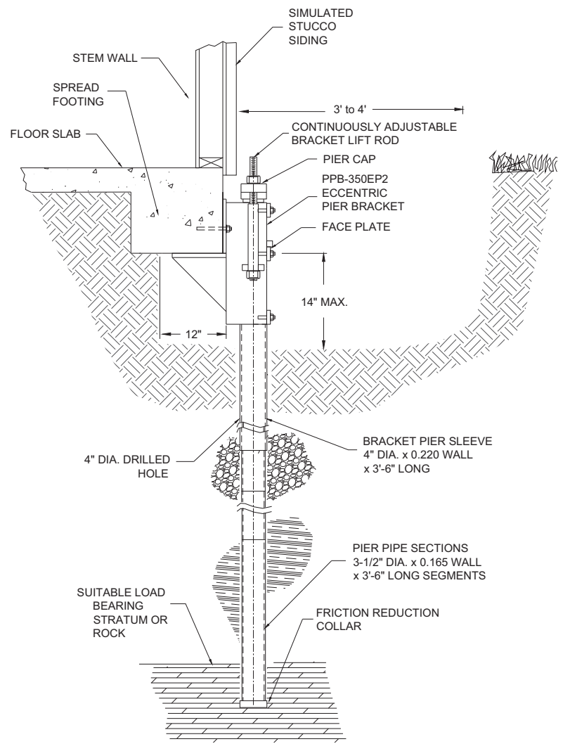
PPB-350EP2 - 2" Eccentric Utility Bracket Application Drawing
