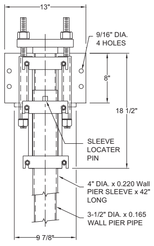
PPB-350EP2 - 2" Eccentric Utility Bracket Details
